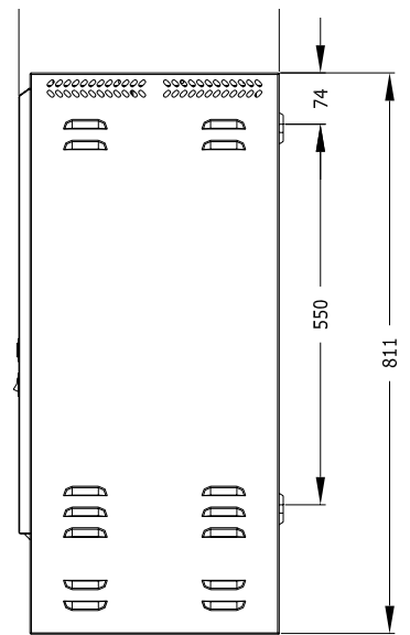
Below: Side View showing wall mounting points.
